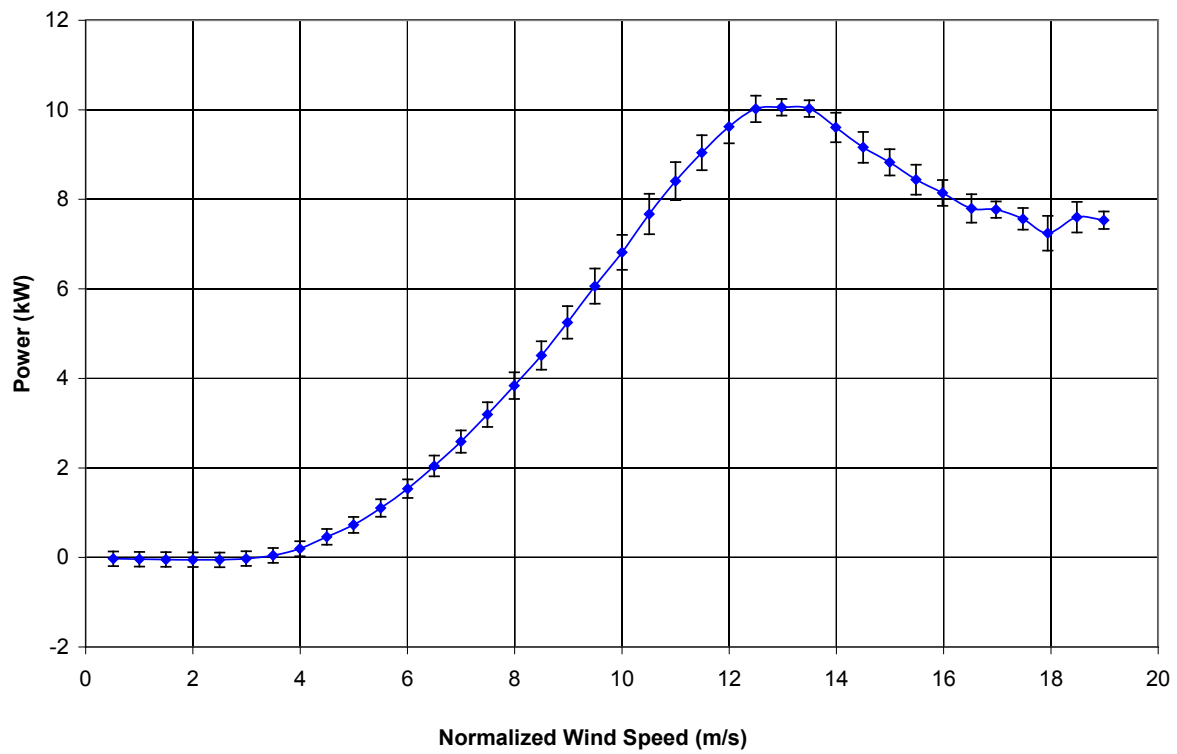
Figure 7. Power curve at site average density; 1.05 kg/m 3
