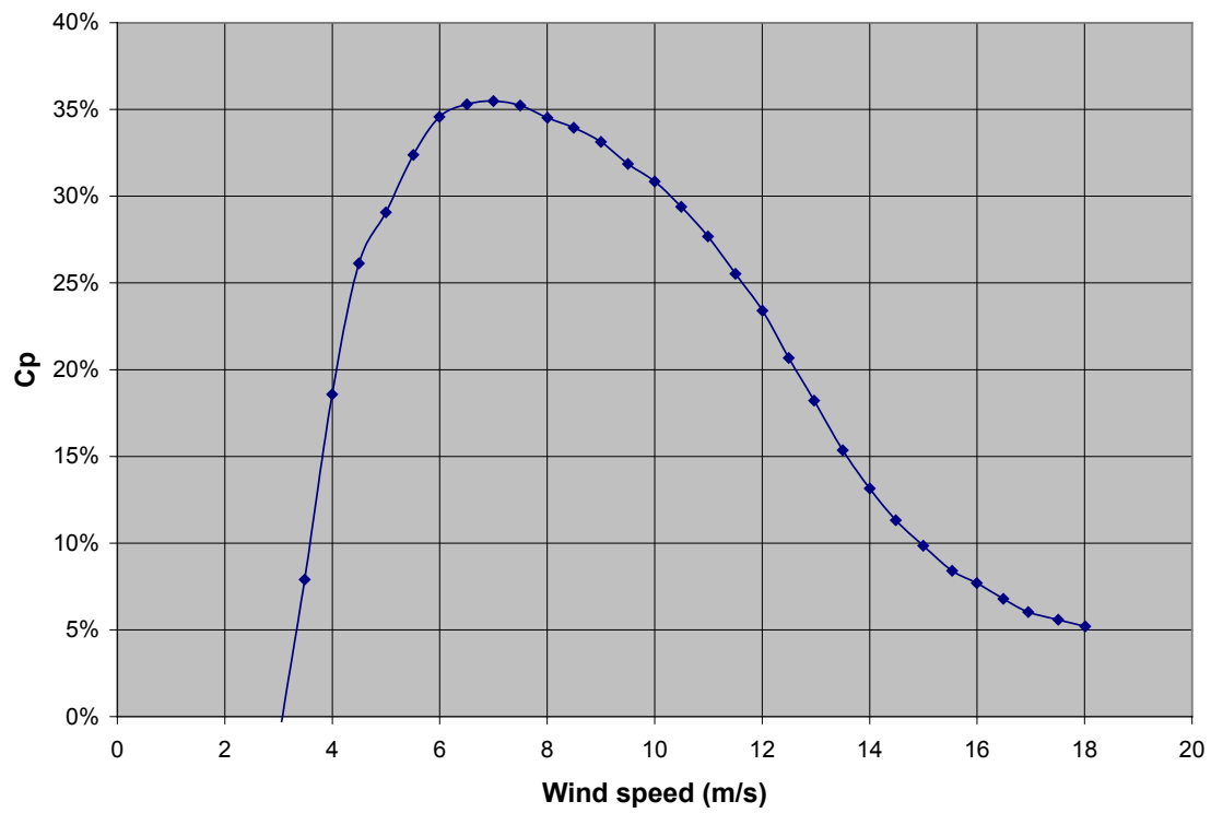
Figure 9. Coefficient of performance at sea level density; 1.225 \text{ kg/m}^3
